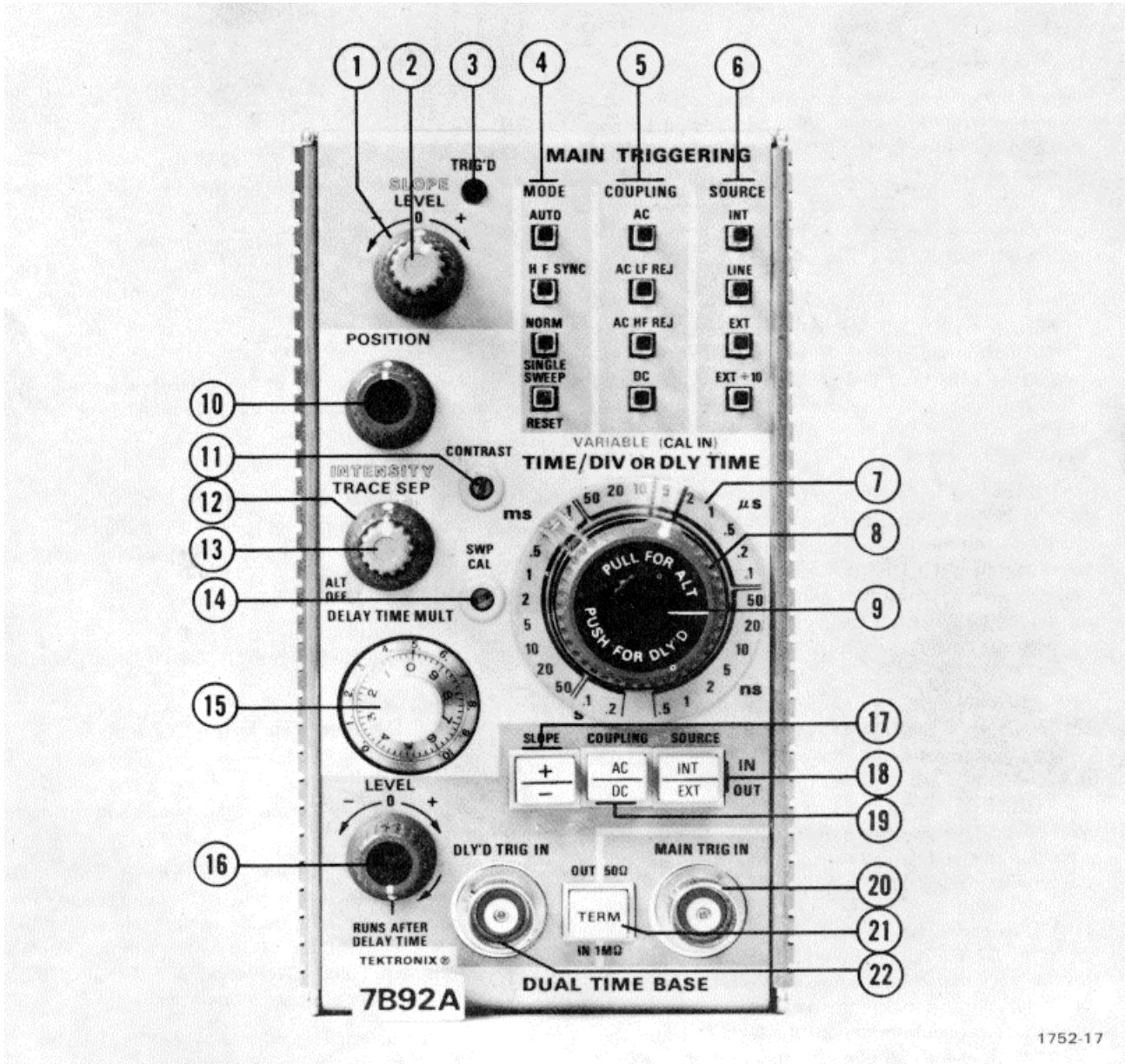
Figure 2-3. Front-panel controls and connectors
