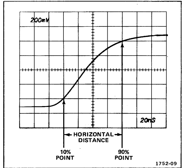
Figure 2-8. Measuring risetime.
