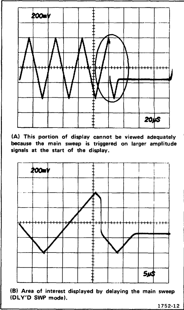
Figure 2-11. Displaying a complex signal using delayed sweep.
