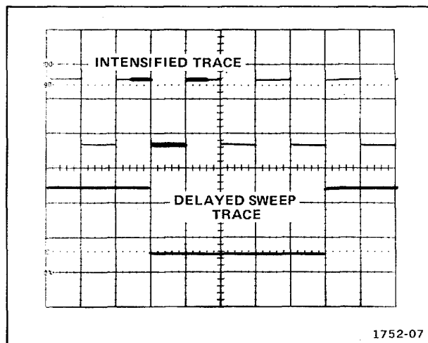
Figure 2-6. Typical alternate sweep display.
