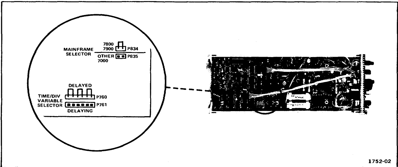
Figure 2-1. Location of Variable and Mainframe Selector multi-pin connectors.
