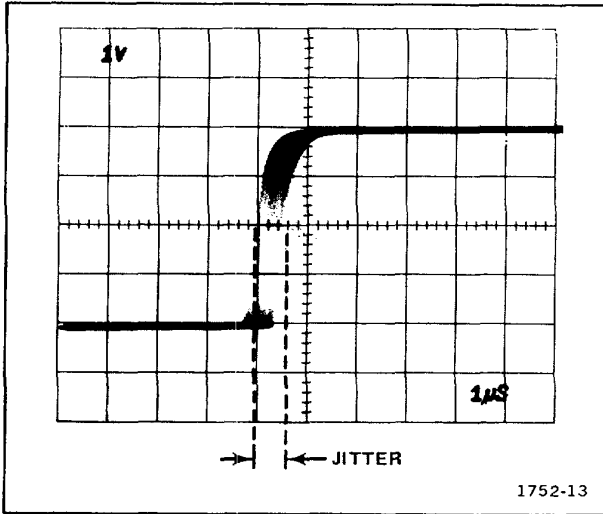
Figure 2-12. Measuring pulse jitter.
