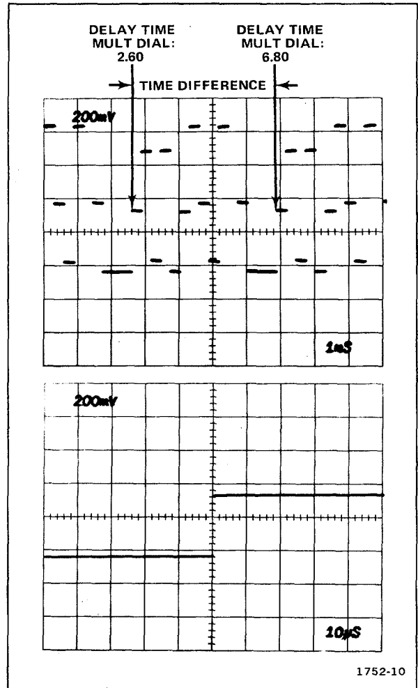
Figure 2-9. Measuring time difference using delayed sweep.
